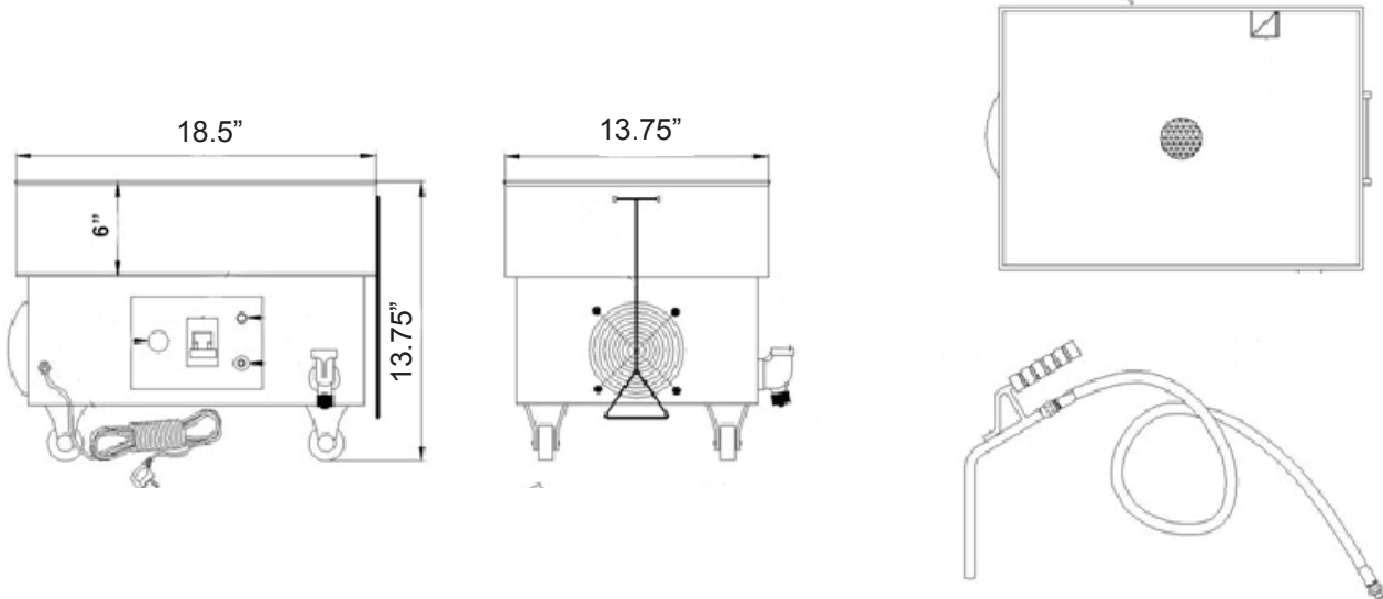
Filtering hose is 5' long with a 1' nozzle
